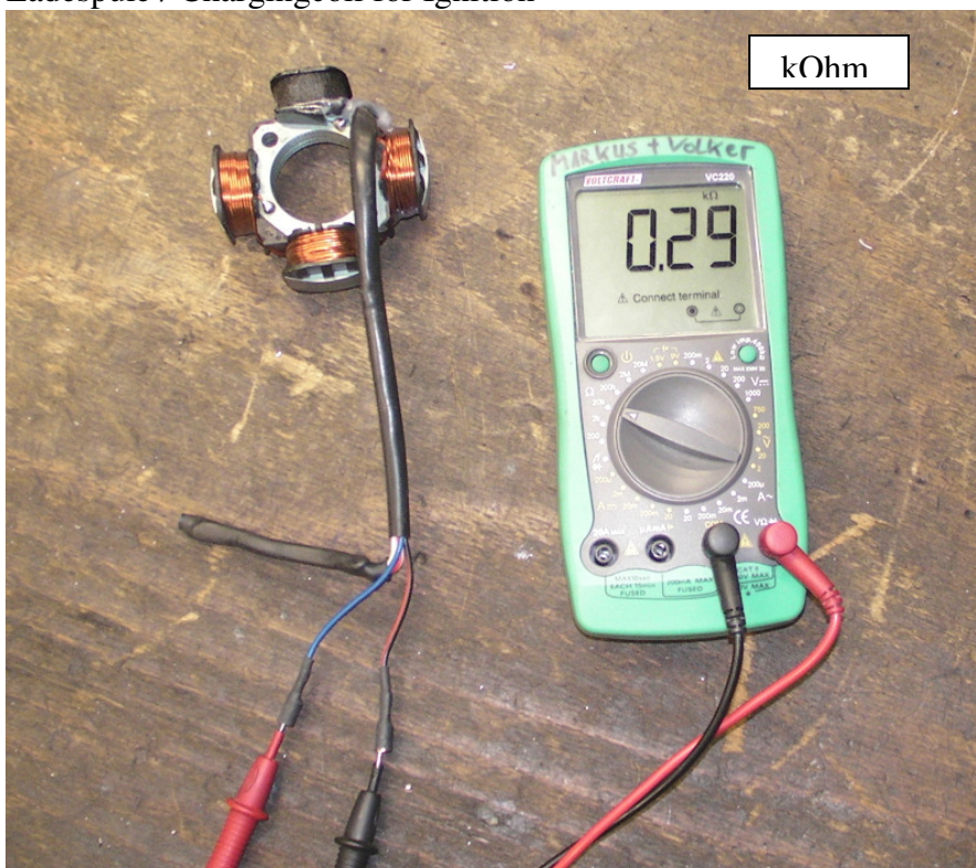
Ladespule / Chargingcoil for Ignition
