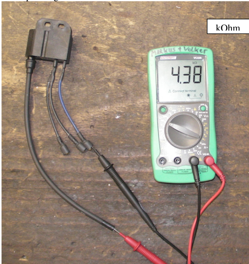
Ladespule / Chargingcoil for Ignition
